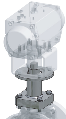
ISO - flange - support tube
